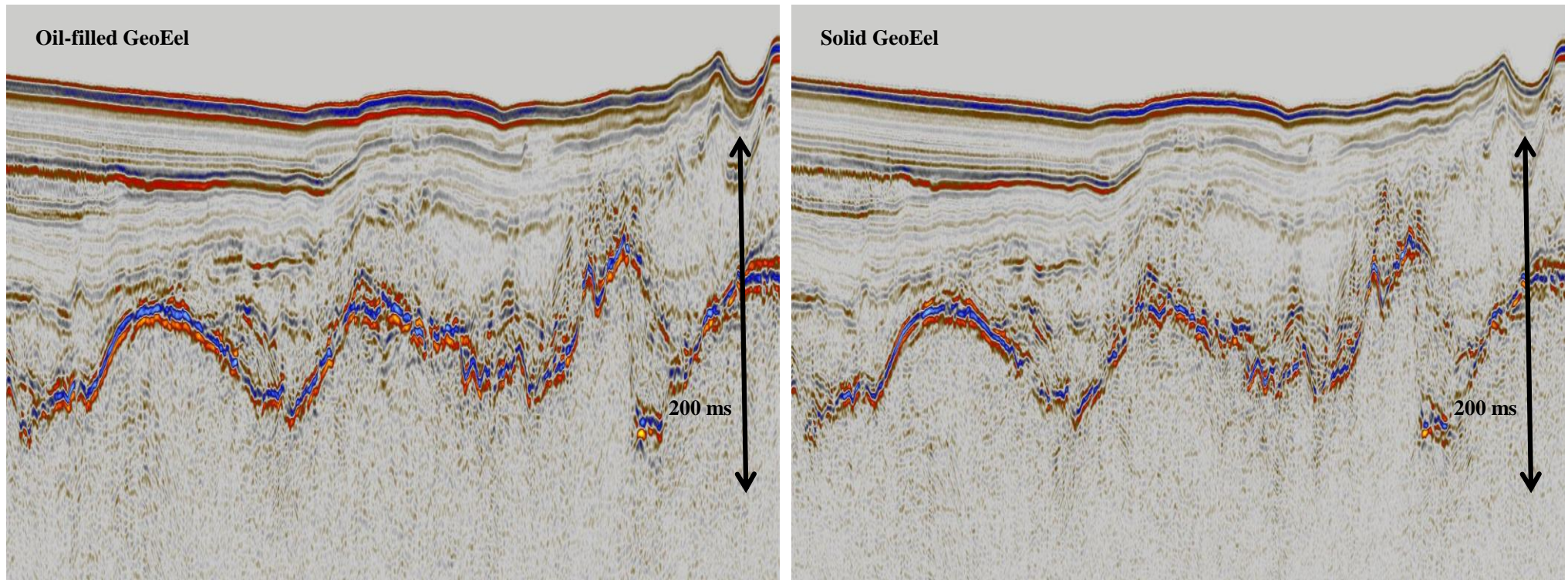
Figure 2: Comparison between Geometrics GeoEel Liquid and solid multi-channel digital streamers. Data collected in the Barents Sea.
