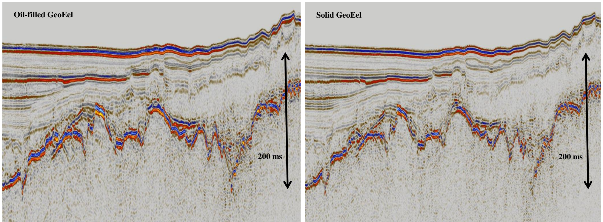
Figure 1: Comparison between Geometrics GeoEel Liquid and solid multi-channel digital streamers. Data collected in the Barents Sea.
