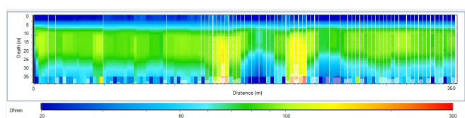
Blocky Inversion of processed Loupe data showing a solution feature in the chalk downs, Southern Britain. Data courtesy of Terradat
