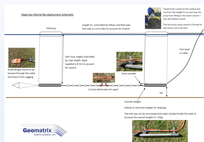
Syscal Deep Marine deep tow deployment
