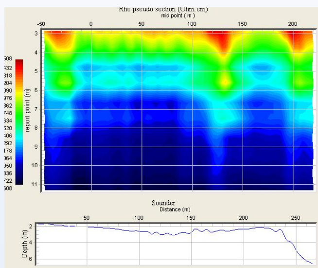
Example Marine Resistivity dataset from a fresh water lake.
