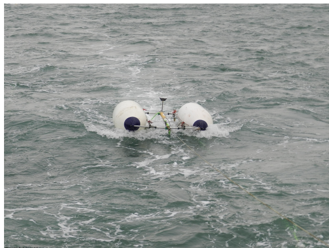
LF Bubble Pulser seismic source undertow with GPS mounted on central spar.
