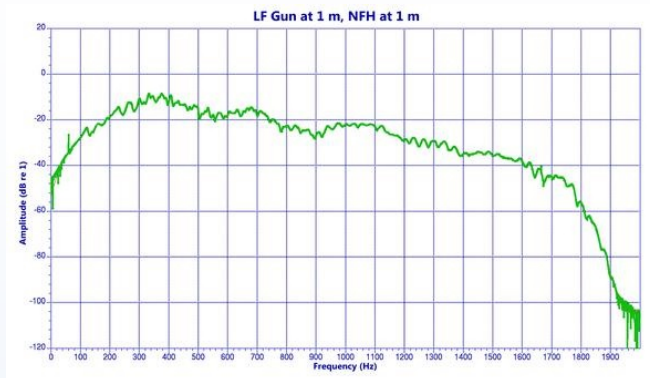
Bubble Pulser LF frequency spectrum
