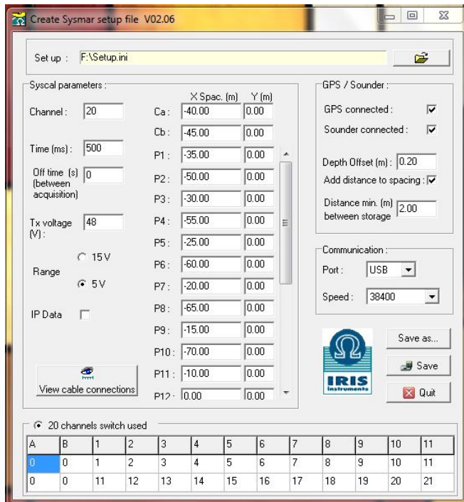
Typical configuration file for a saline marine survey with 20 channels and 5m electrode interval.
